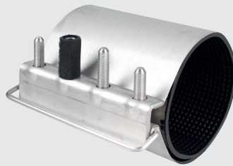
120-00G Repair clamp of stainless steel, multiple tensioned
