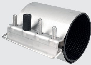
110-00G Repair clamp of stainless steel, single tensioned
