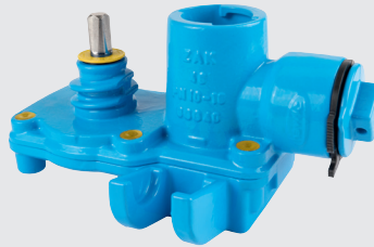
244-00G Hawlinger with horizontal ZAK® socket in pipe direction
