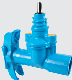
270-01G Valve saddle with ZAK® outlet
