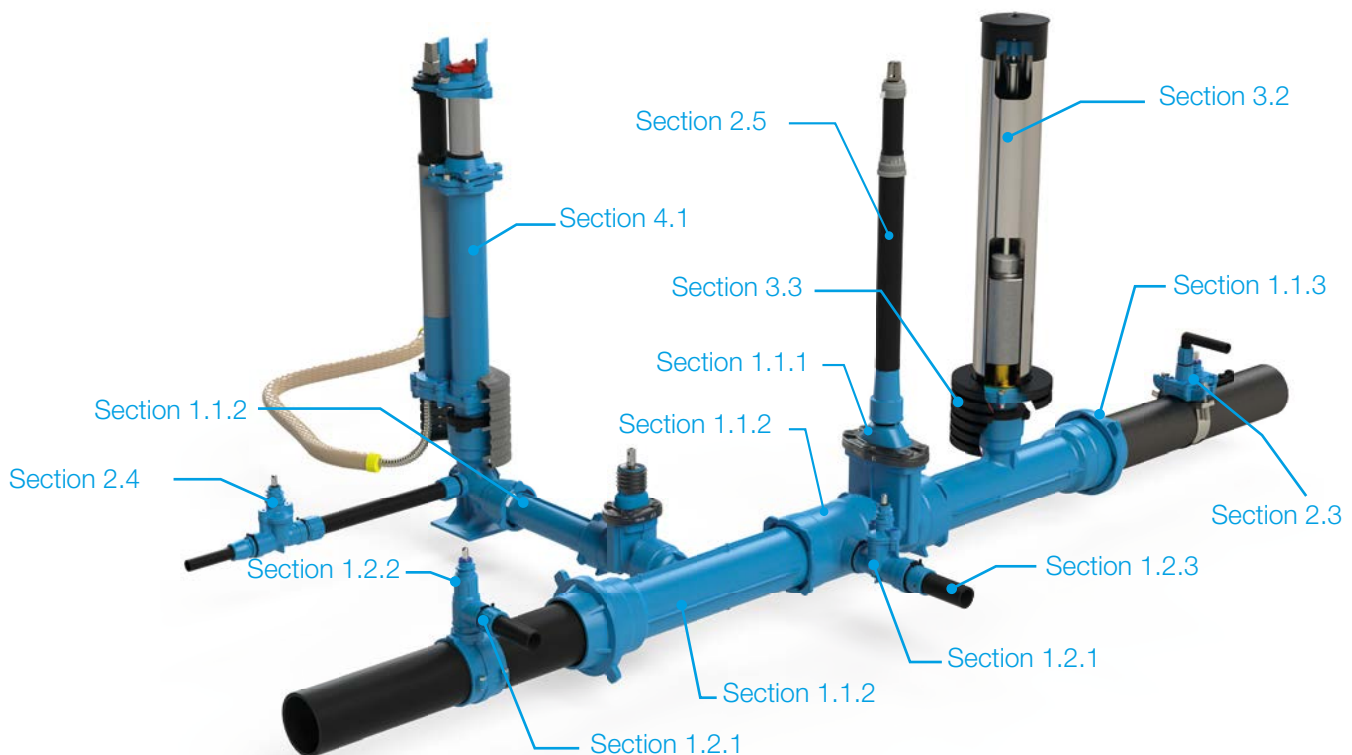
Design of a threadless connection system with a main line and two service lines.
