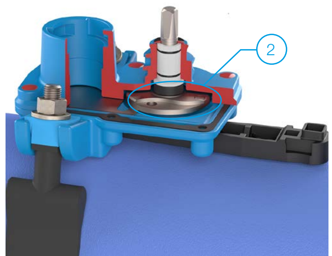
2. Closed position with opened drainage mechanism
