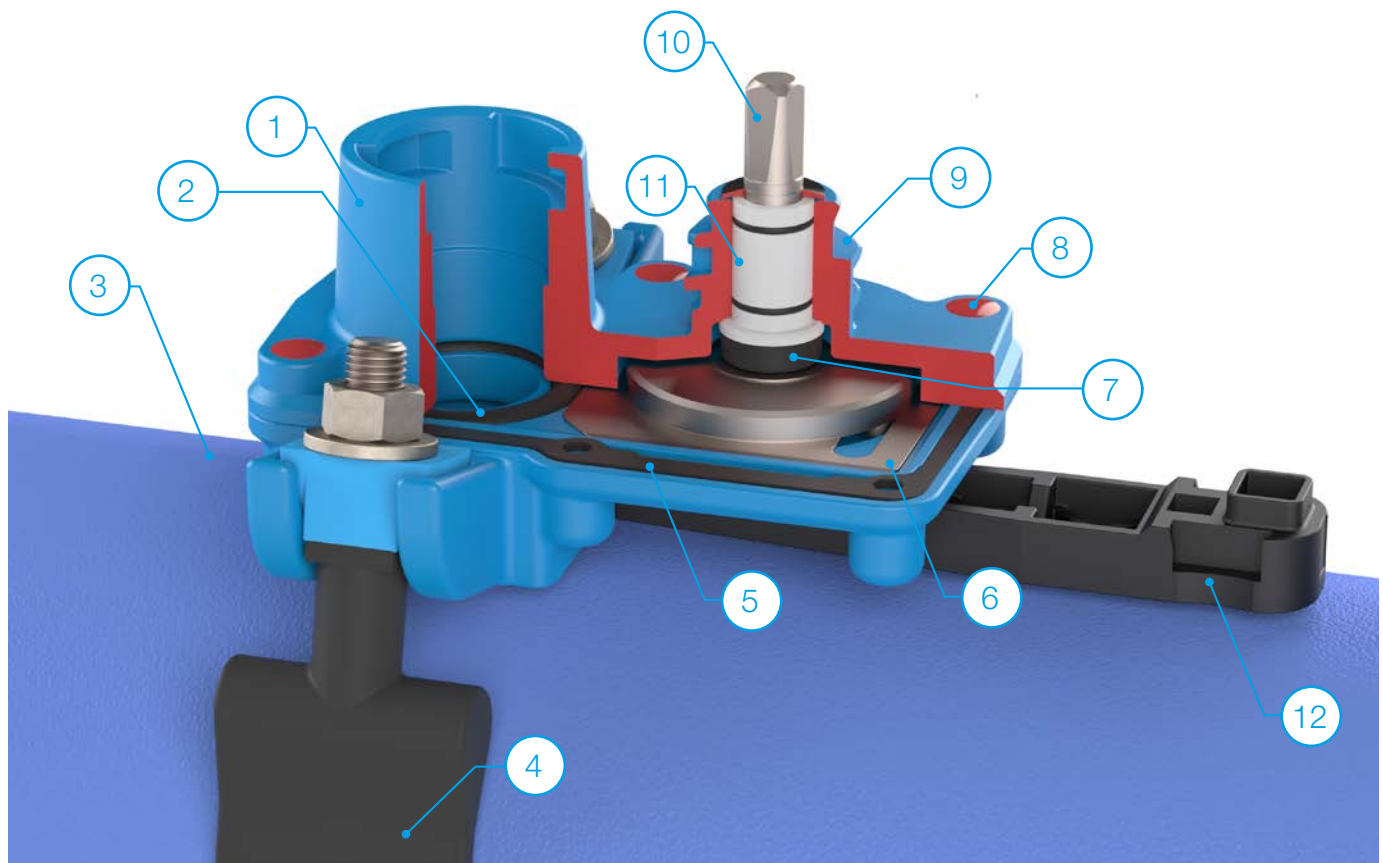
Figure: Pipe drilling saddle type Hawlinger® for CI, steel, and AC pipes with upper ZAK® outlet. (Alternatively also available with threaded outlet.)
