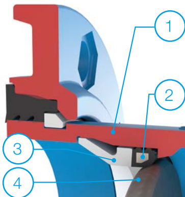
Section view of sealing system
