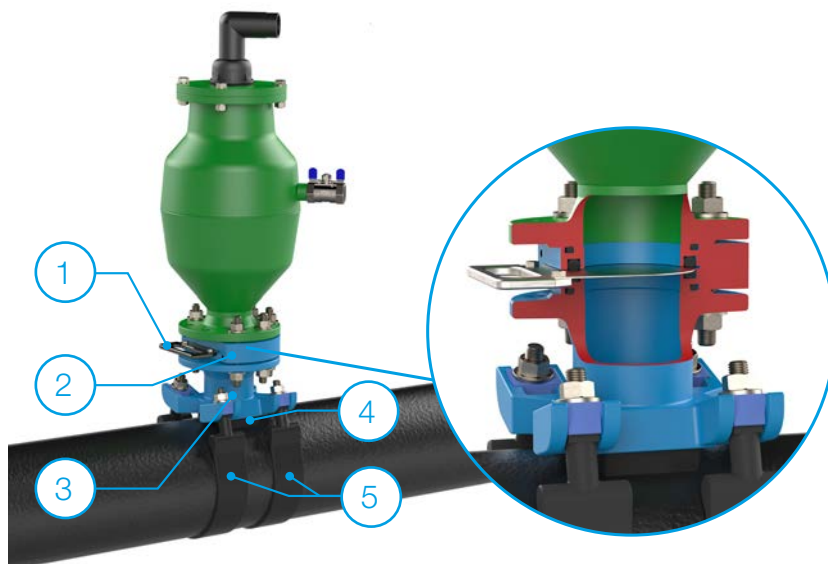
Double strap saddle with flange outlet (Ord. No. 359F)
