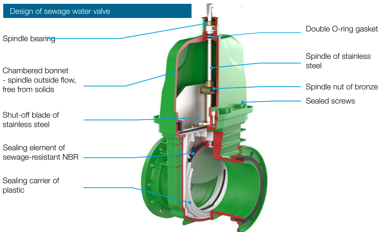
Figure: Sewage water gate valve DN 250 with loose flanges
