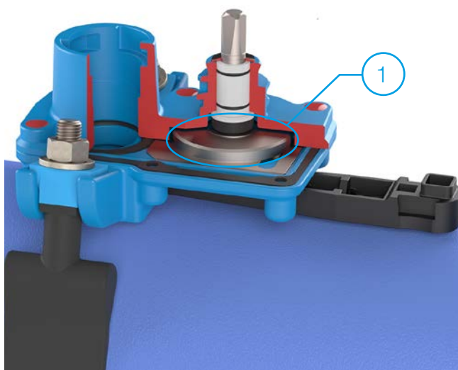
1. Opened position with closed drainage mechanism (shut-off blade outside the flow)
