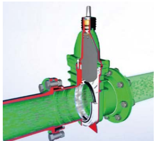
Sewage water gate valve opened (DN 200)
