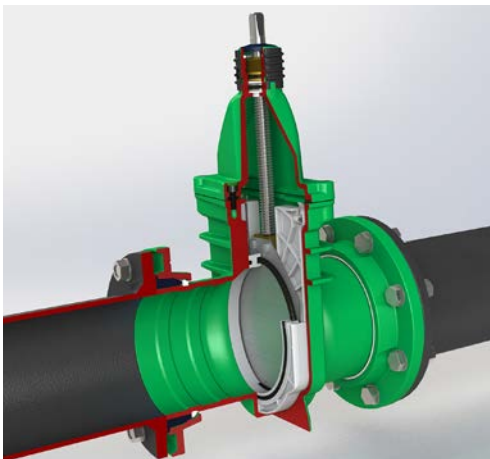
Sewage water gate valve closed (DN 200)
