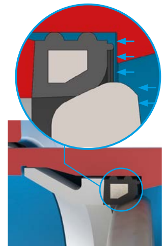
Functional principle 2
